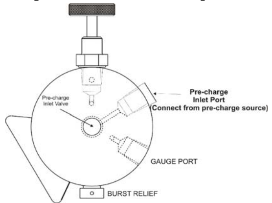
Figure - 3 Pre-Charge End Cap Detail
